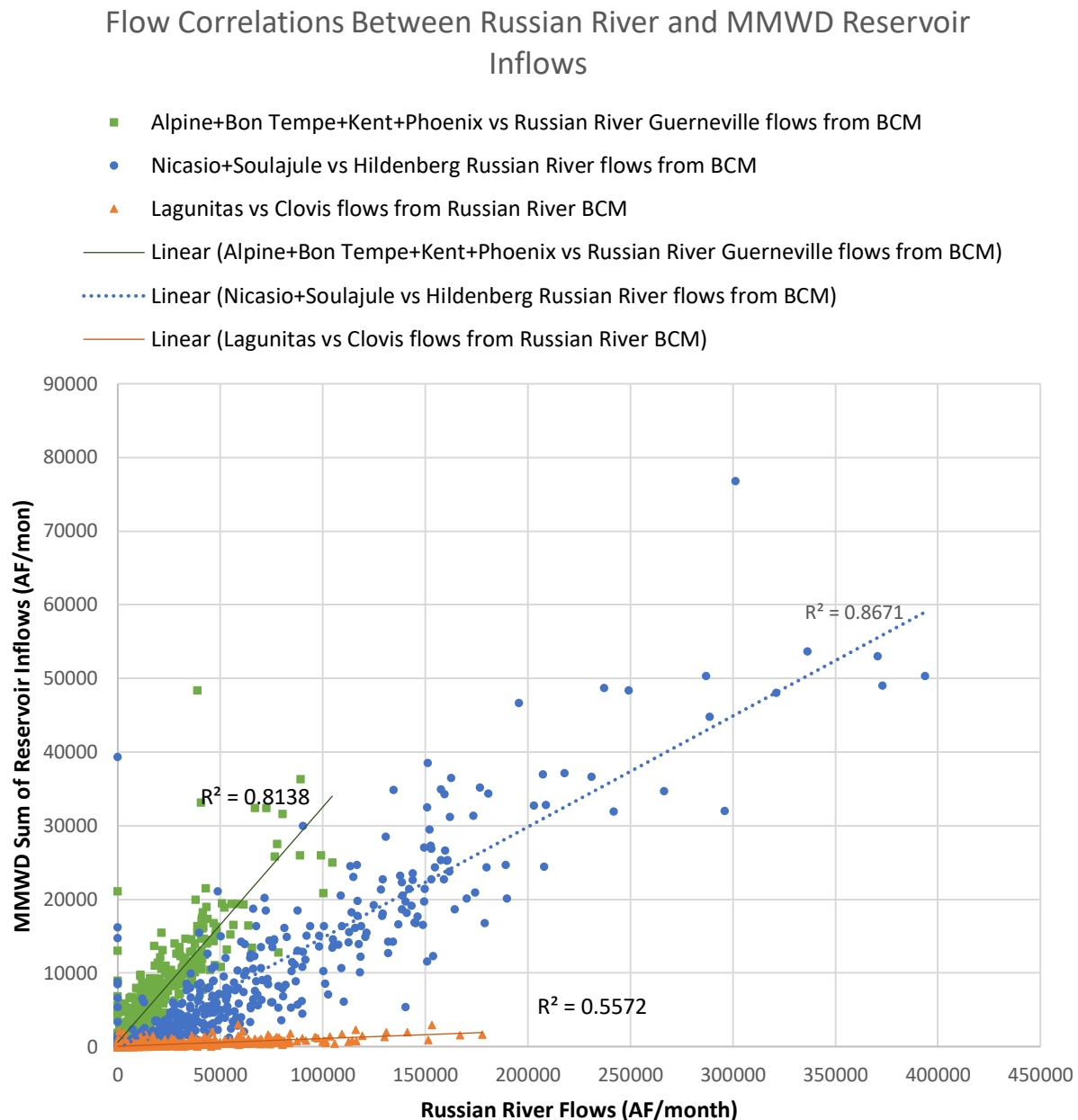
Figure B-6. Monthly correlation of flows between inflows MMWD's reservoirs versus Russian River BCM flow locations
