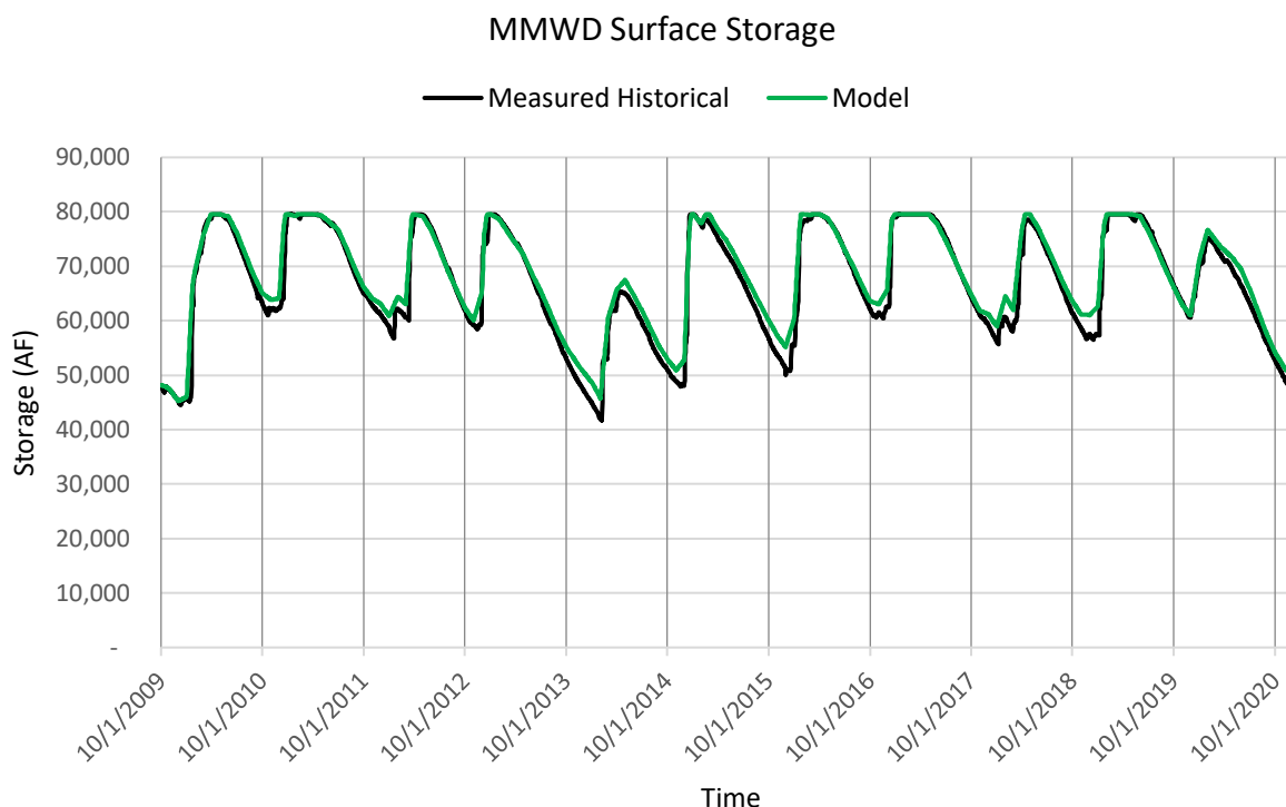
Figure B-7. MMWD total storage comparison between model results and measured storage for the model validation period
