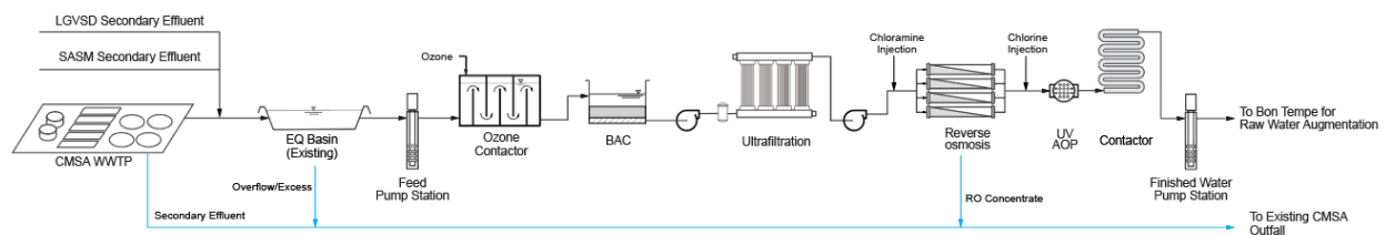
Figure C-25. DPR purified water treatment train
