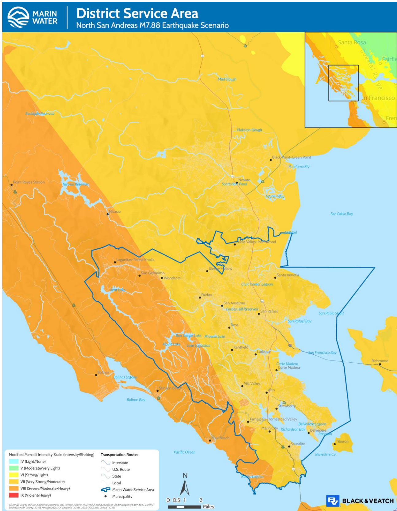
Figure 8-6. North San Andreas M7.88 Earthquake Scenario
