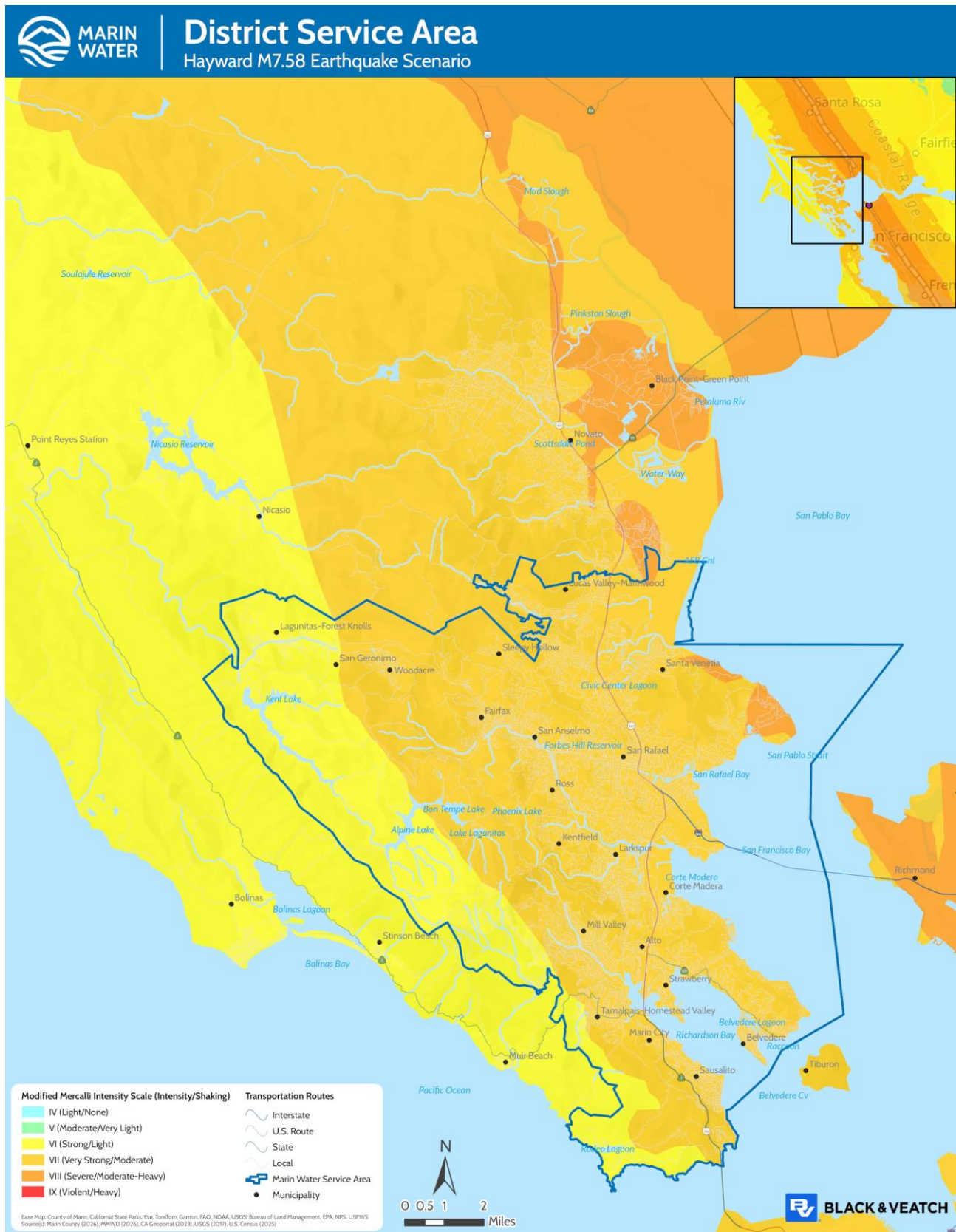
Figure 8-5. Hayward/Rodgers Creek M 7.58 Earthquake Scenario
