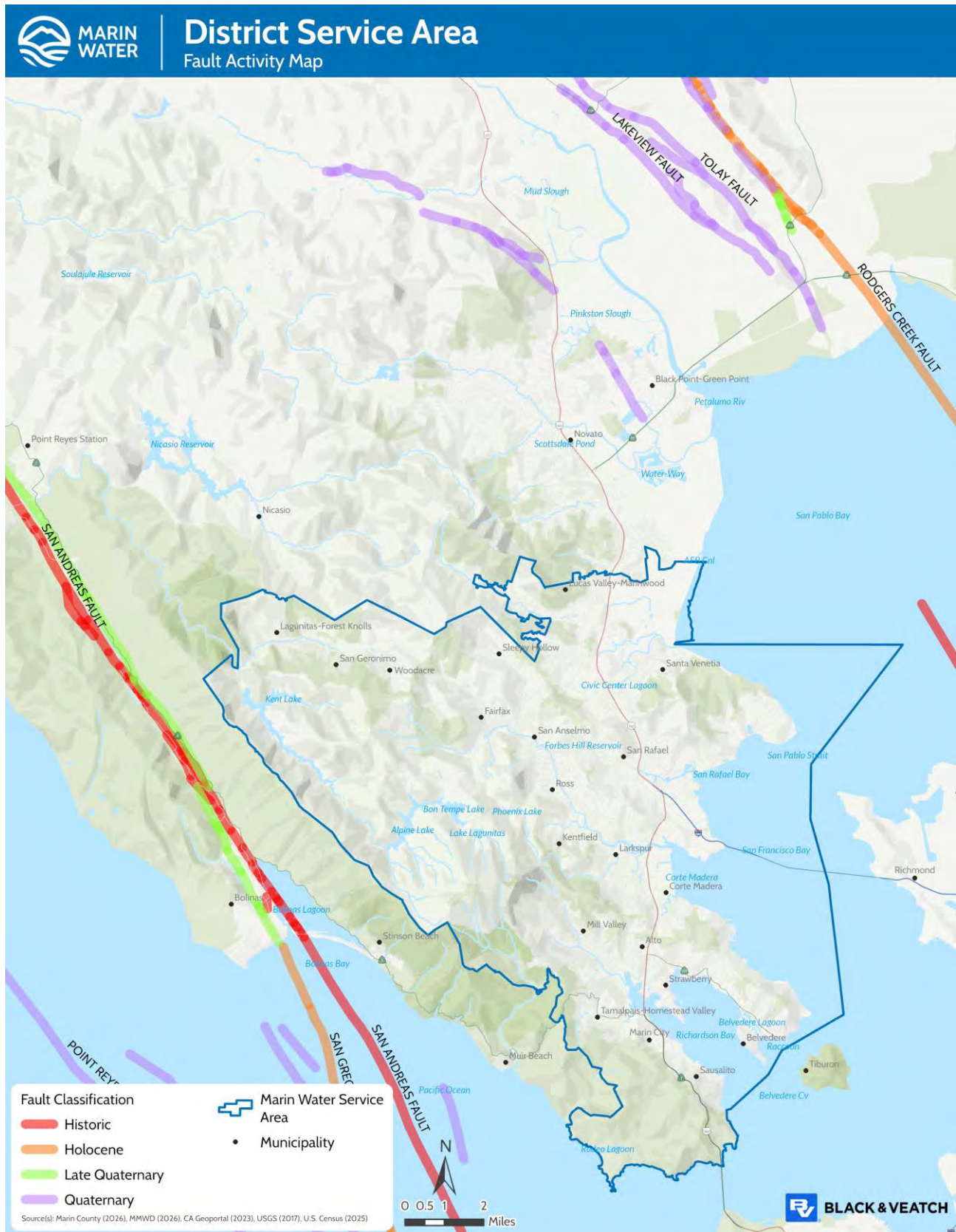
Figure 8-2. Earthquake Fault Zones Near the Planning Area
