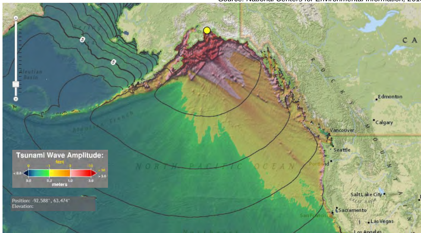
Figure 14-3. 1964 Alaska Earthquake Tsunami Event
