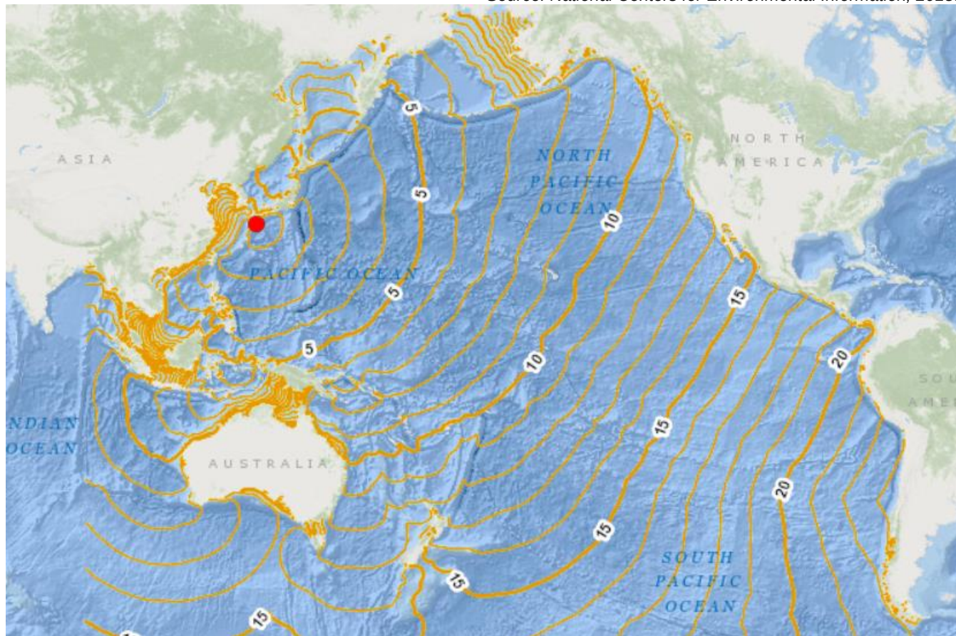
Figure 14-5. Potential Tsunami Travel Times in the Pacific Ocean, in Hours
