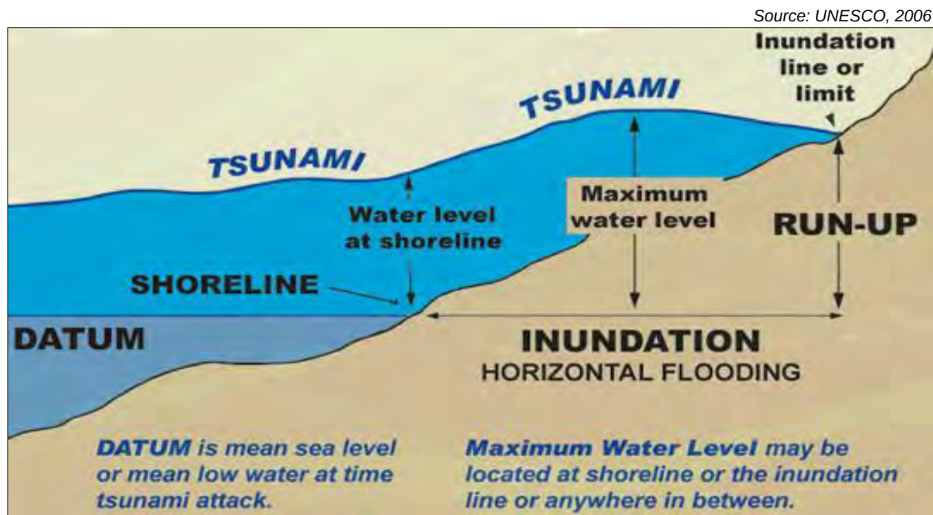
Figure 14-2. Runup Distance and Height in Relation to the Datum and Shoreline
