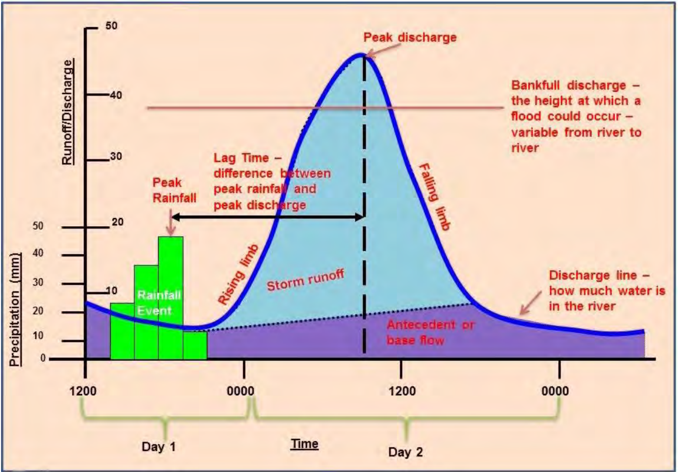
Figure 10-2. Example Hydrograph
