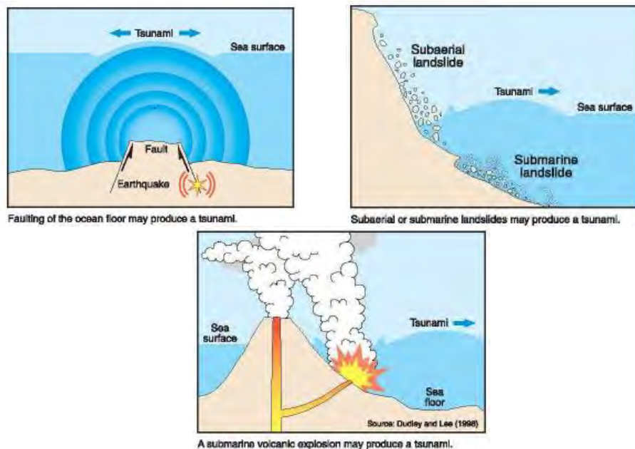
Figure 14-1. Common Sources of Tsunamis
