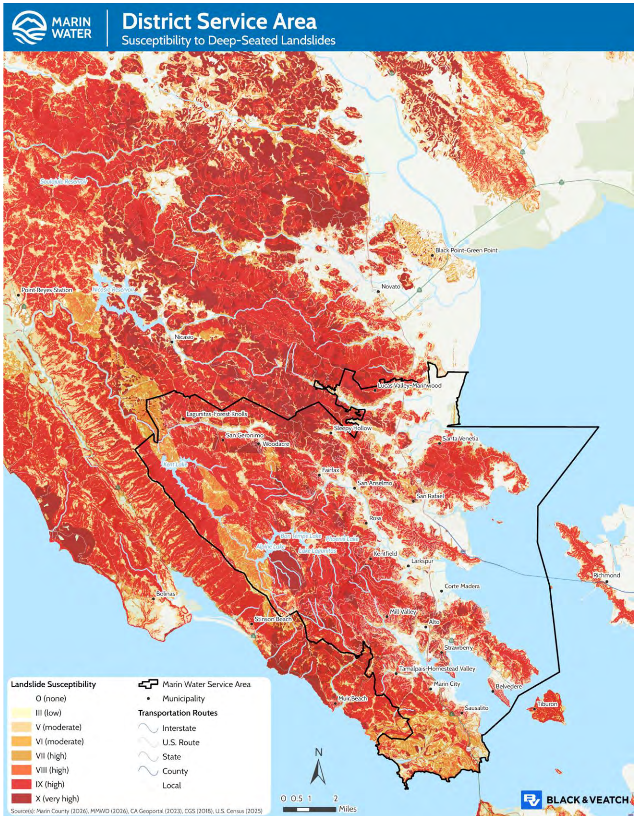
Figure 12-2. Susceptibility to Deep-Seated Landslides
