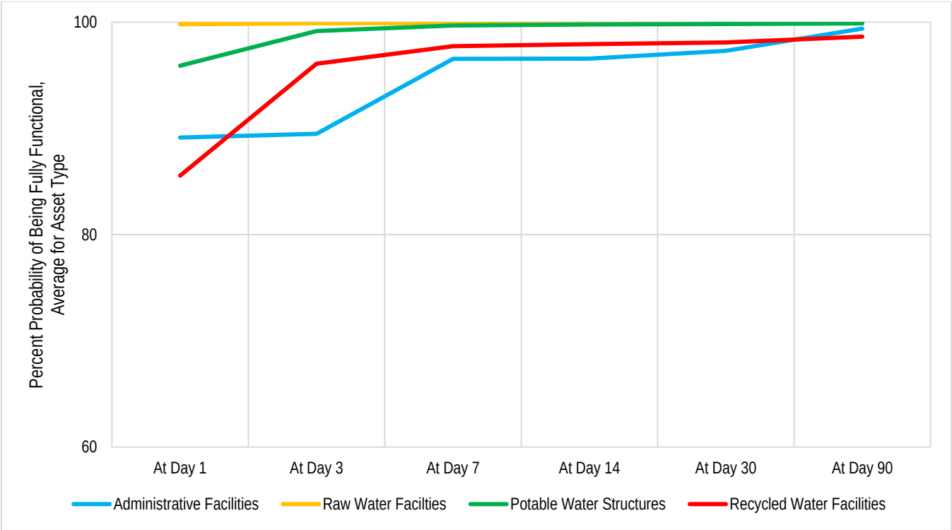
Figure 8-12. Average Probability of Full Functionality After West Napa M6 Event
