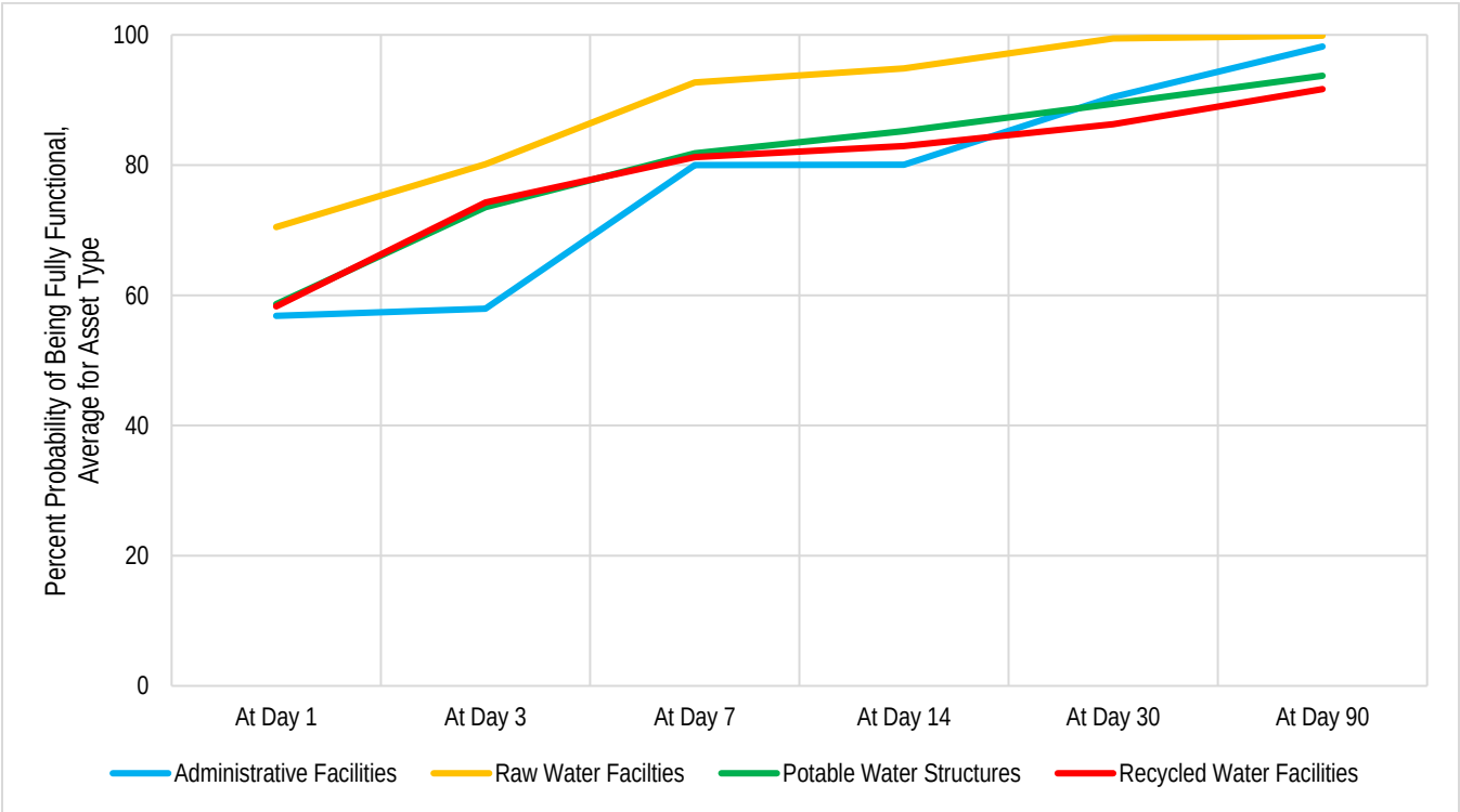
Figure 8-13. Average Probability of Full Functionality After 100-Year Probabilistic Event
